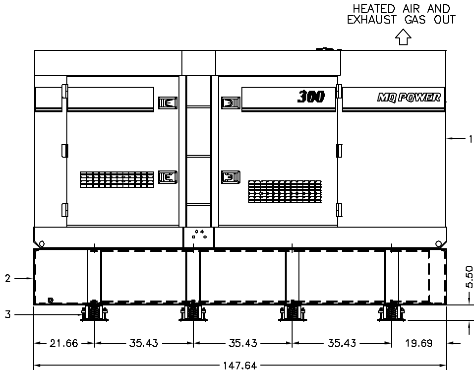
SIDE VIEW
