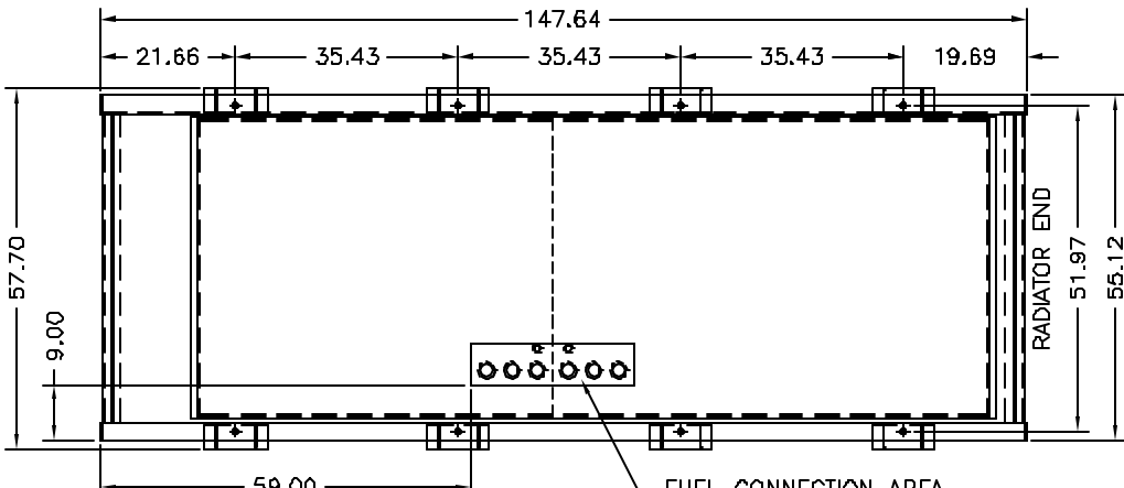
TOP VIEW OF 470GAL. SUBBASE TANK WITH RUPTURE BASIN & STUB-UP
