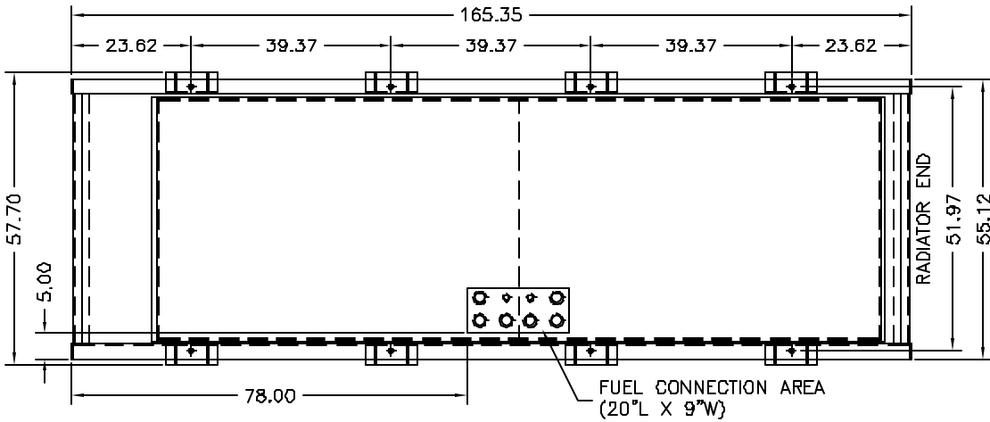
TOP VIEW OF 540GAL. SUBBASE TANK WITH RUPTURE BASIN & STUB-UP
