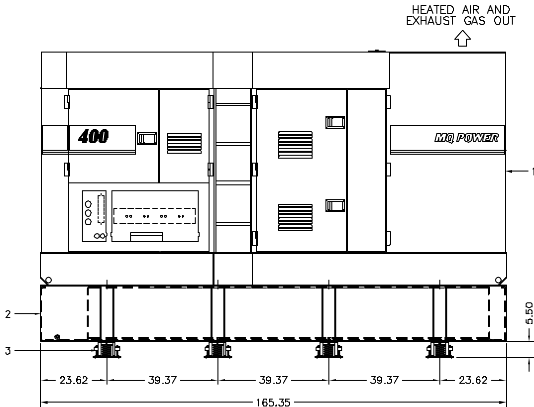
SIDE VIEW
