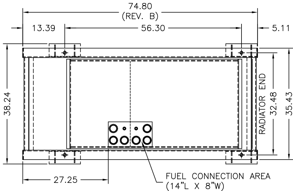
TOP VIEW OF 80GAL. SUBBASE TANK WITH RUPTURE BASIN & STUB-UP
