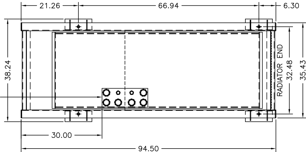
TOP VIEW OF 110GAL. SUBBASE TANK WITH RUPTURE BASIN & STUB-UP
