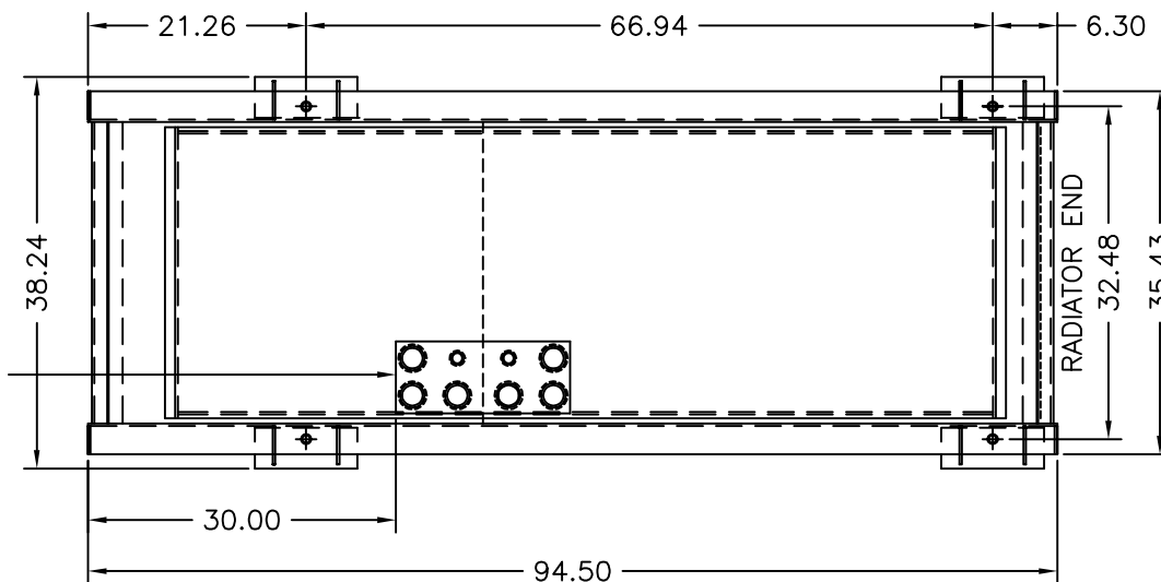
TOP VIEW OF 120GAL. SUBBASE TANK WITH RUPTURE BASIN & STUB-UP
