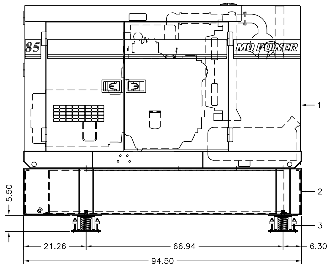
SIDE VIEW
