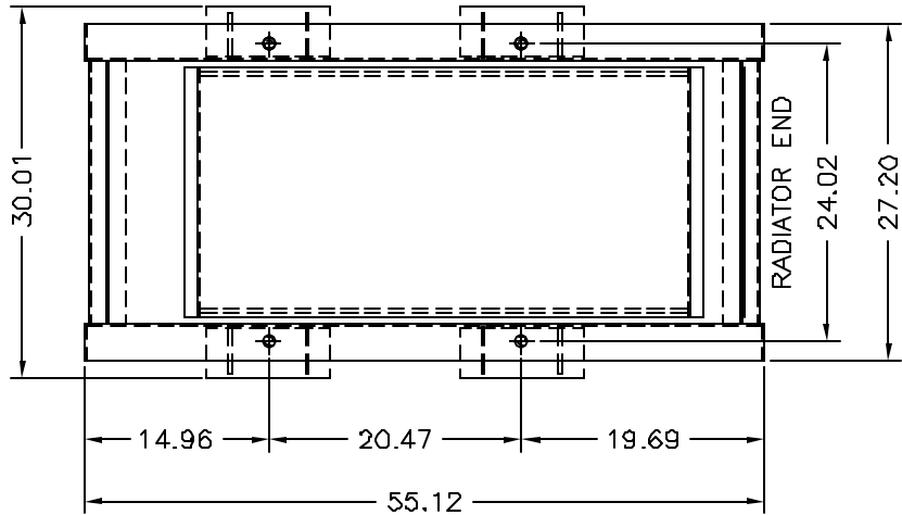
TOP VIEW OF 40GAL. SUBBASE TANK WITH RUPTURE BASIN & STUB-UP
