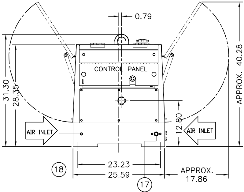
REAR VIEW
