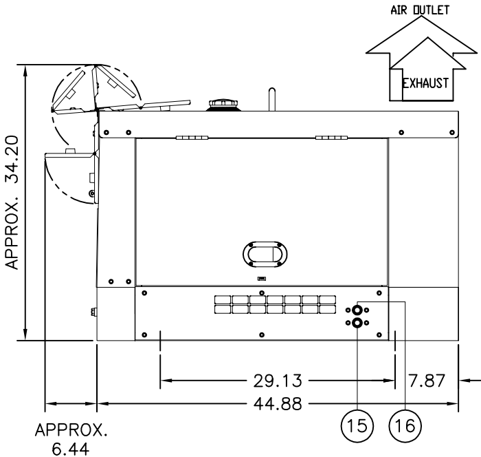
RIGHTSIDE VIEW
