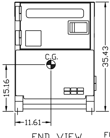
END VIEW
