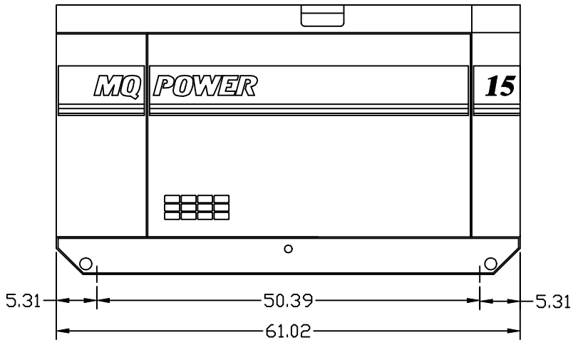
LEFTSIDE VIEW
