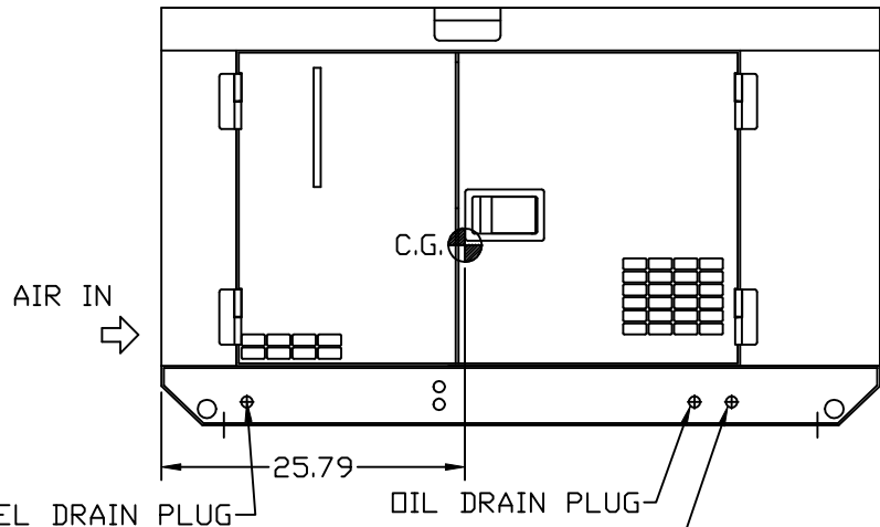
RIGHTSIDE VIEW
