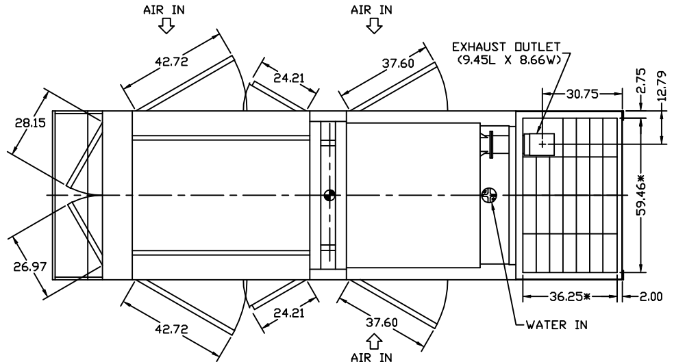
TOP VIEW
