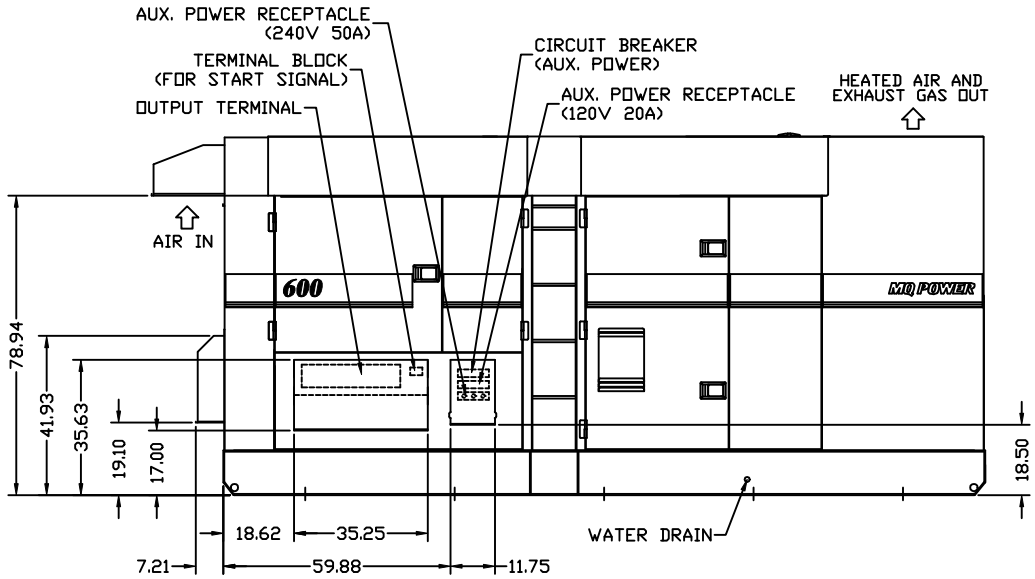
RIGHTSIDE VIEW
