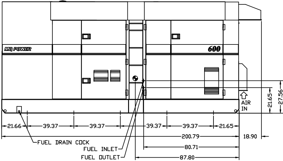
LEFTSIDE VIEW
