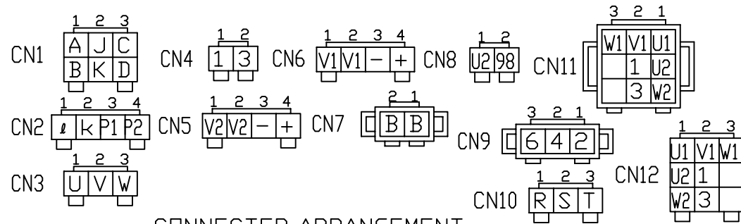
CONNECTER ARRANGEMENT (WIRING VIEW)
