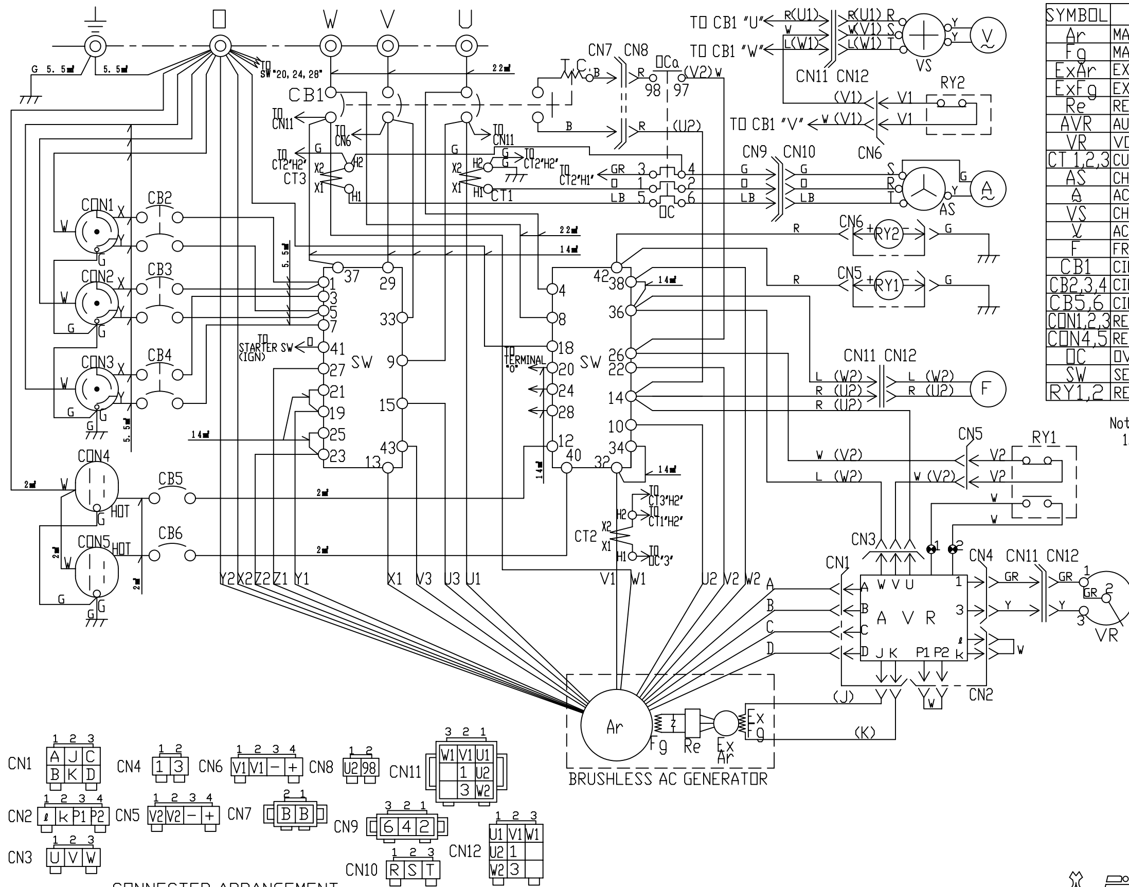
CONNECTER ARRANGEMENT (WIRING VIEW)
