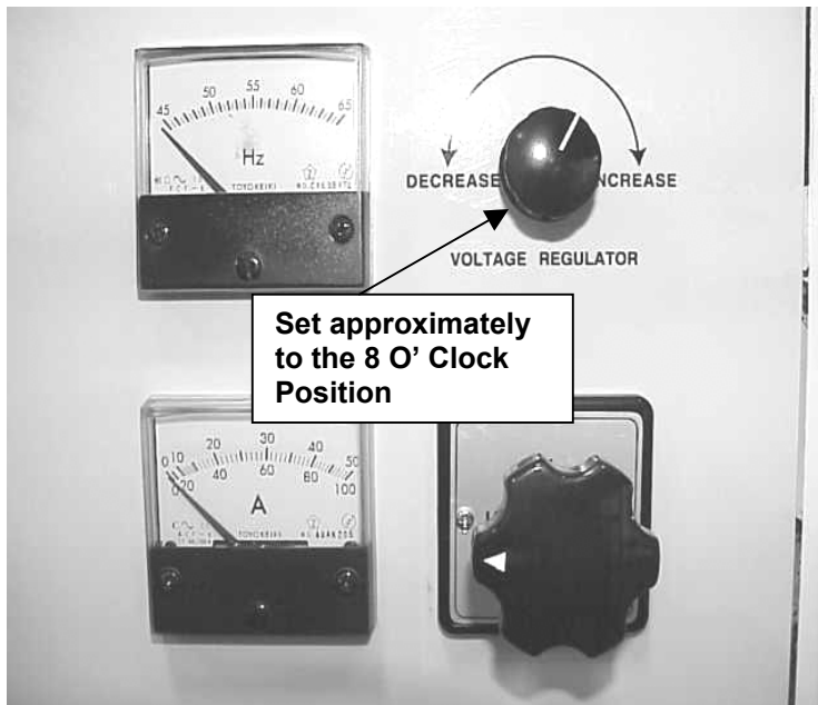
Figure 1 Voltage Regulator Control
