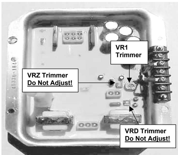
Figure 2 Automatic Voltage Regulator (AVR)
