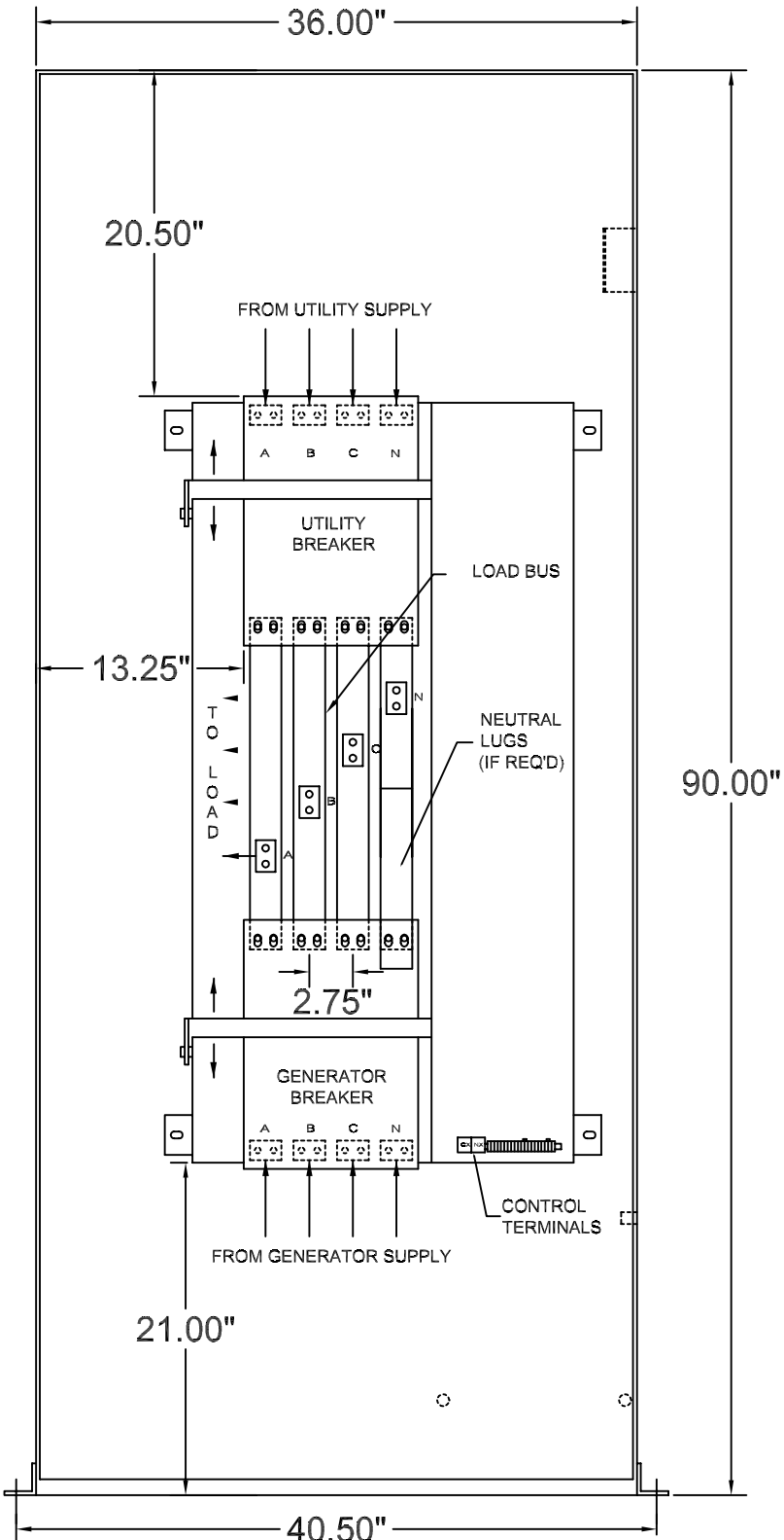
FRONT VIEW DOOR NOT SHOWN
