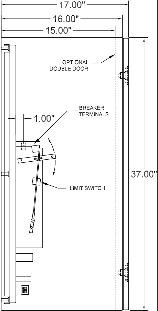
LEFT VIEW
