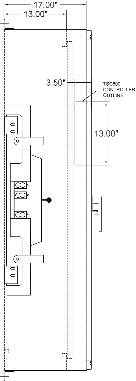
LEFT VIEW
