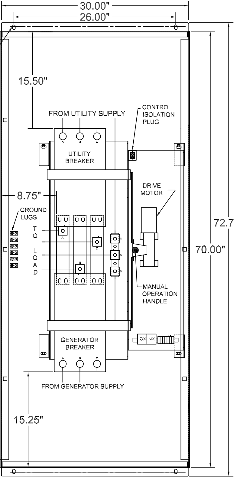
INTERIOR FRONT VIEW (DOOR NOT SHOWN)
