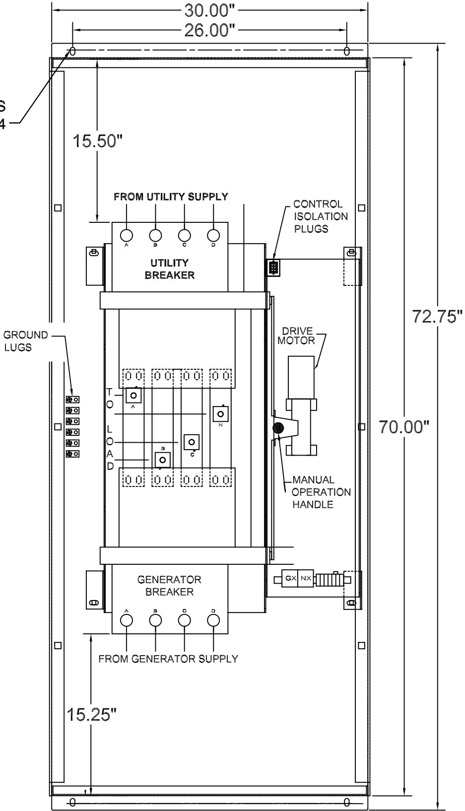
INTERIOR FRONT VIEW (DOOR NOT SHOWN)
