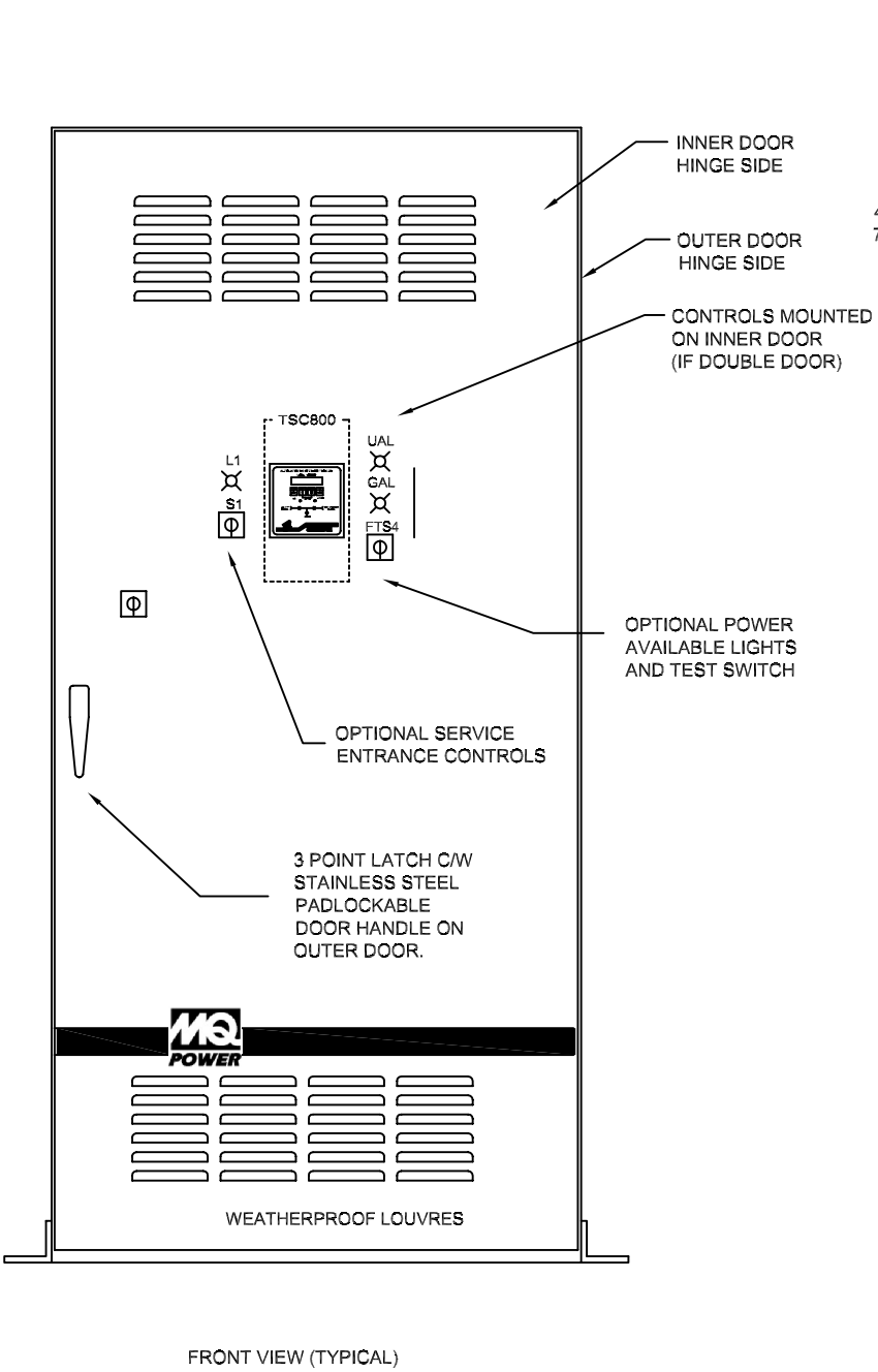
FRONT VIEW (TYPICAL)
