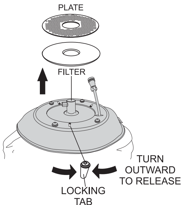
Figure 42. Filter Removal
