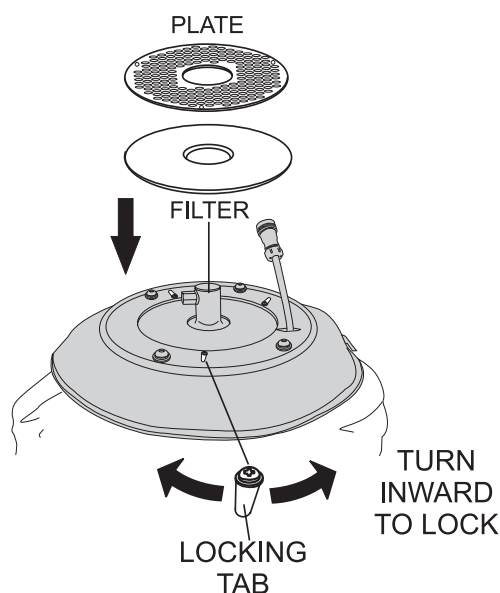
Figure 44. Filter/Plate Install
