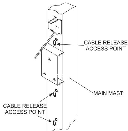
Figure 35. Cable Release Access Point
