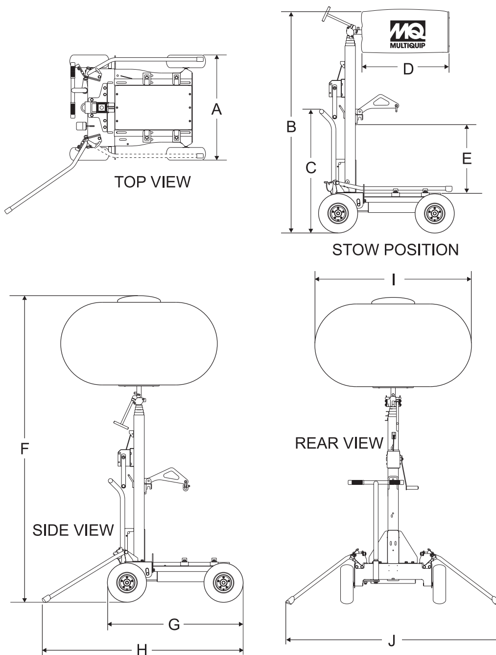
Figure 2. Dimensions
