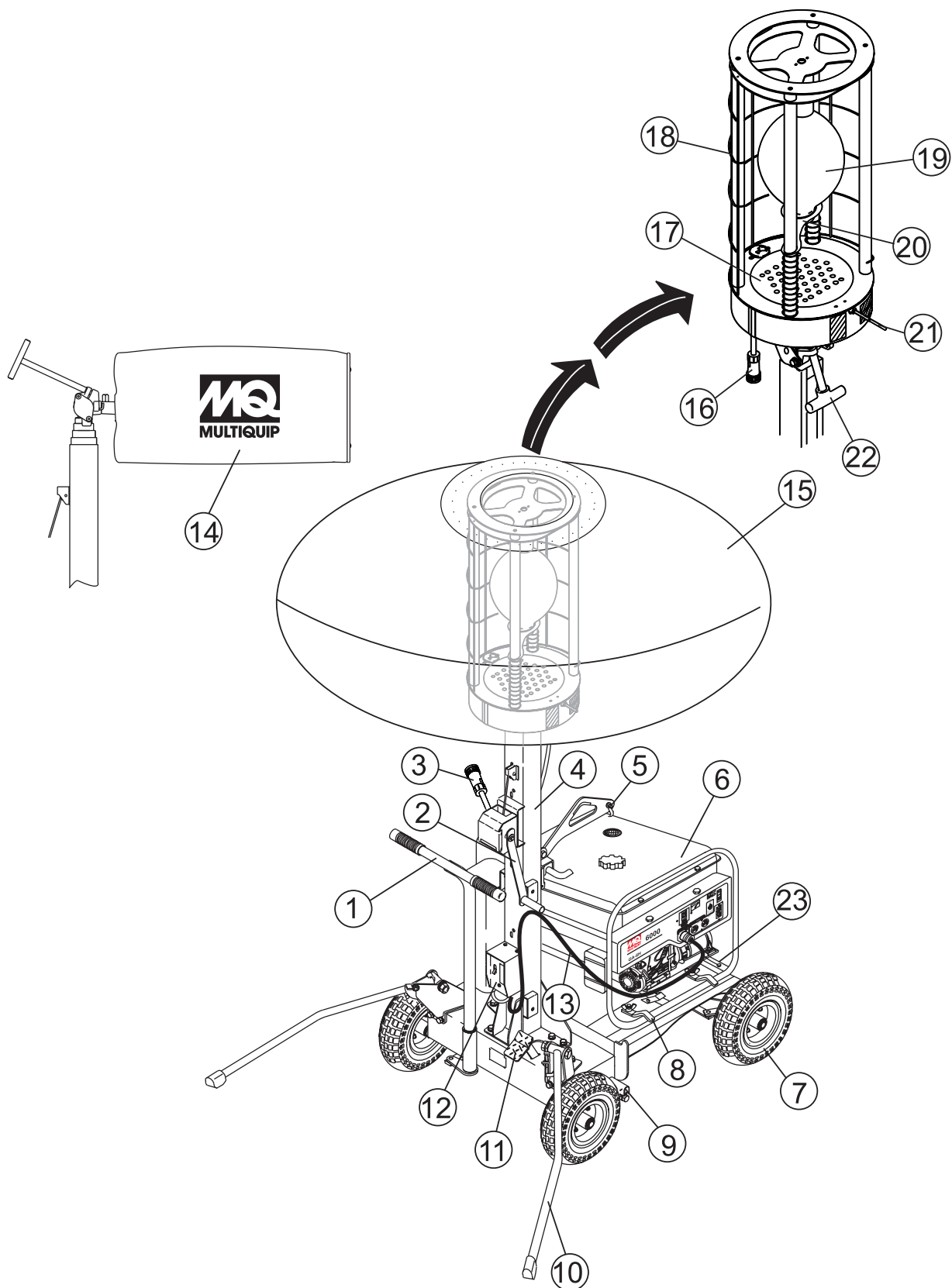
Figure 6. Major Components
