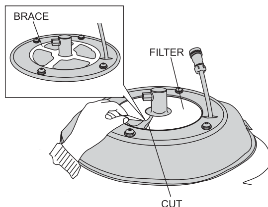
Figure 43. Filter Placement
