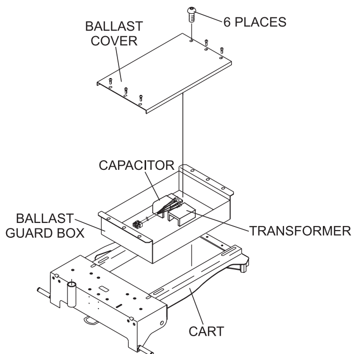
Figure 40. Removing the Ballast
