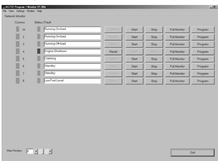
Multi-genset monitor screen (AS732 RS485 systems only)
