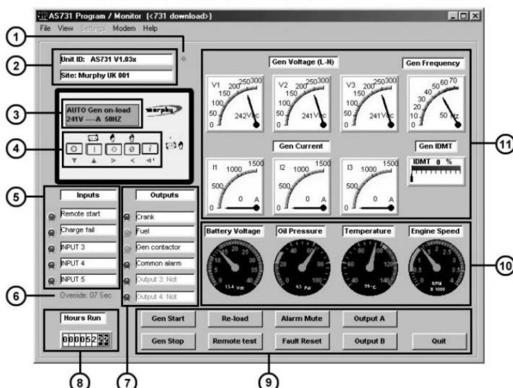
Single genset ('full') monitor screen (all units)
