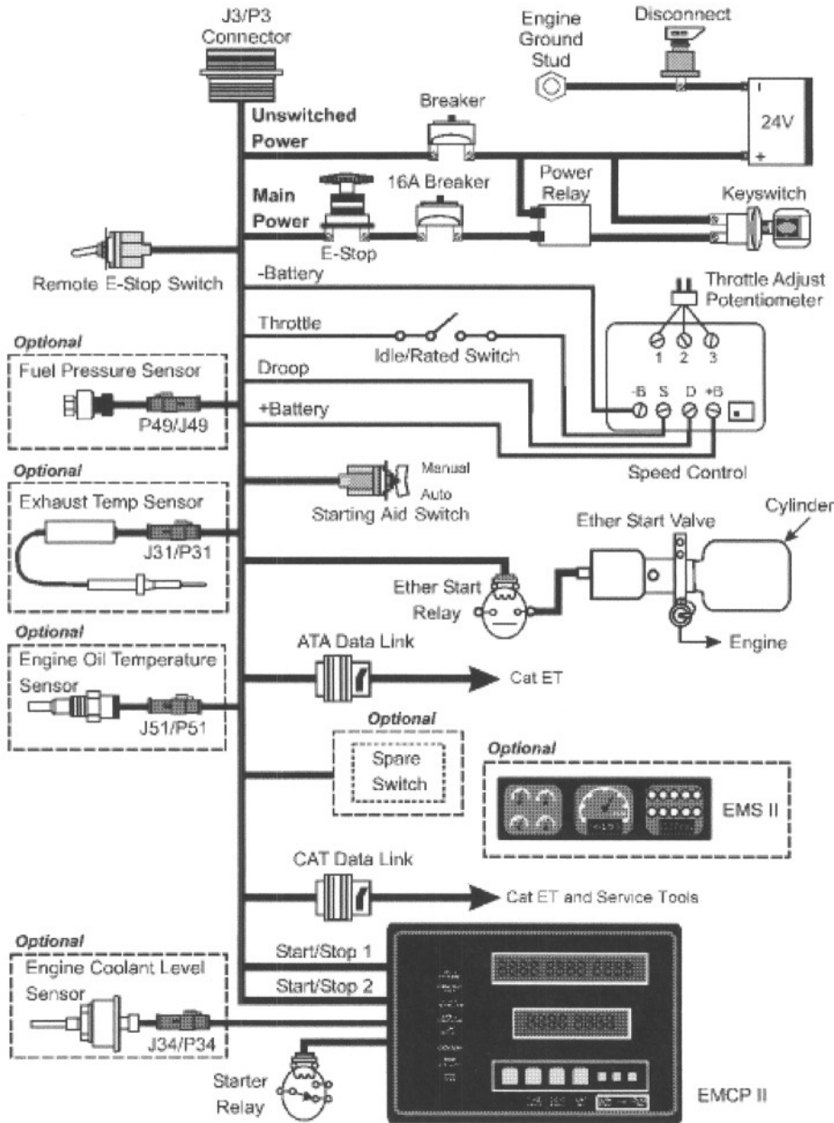
Diagram for Engines with EMCP II
