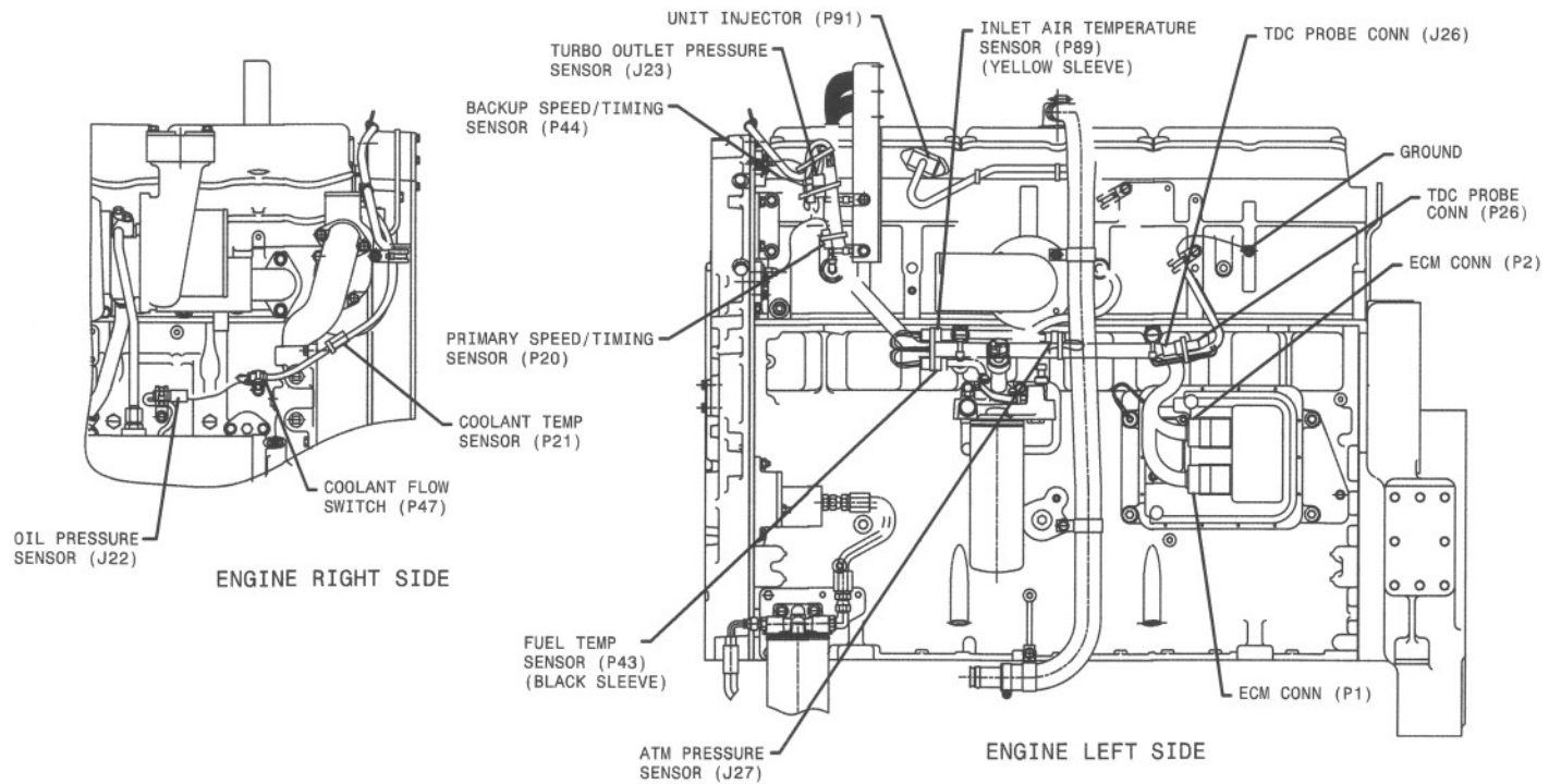
3456 ENGINE COMPONENT LOCATIONS
