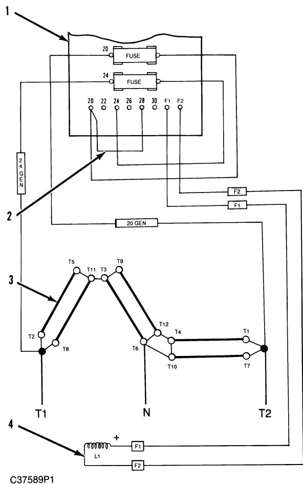
Connection Diagram For Single Phase Sensing (1) VR3 regulator. (2) Jumper. (3) Main stator. (4) Exciter stator.
