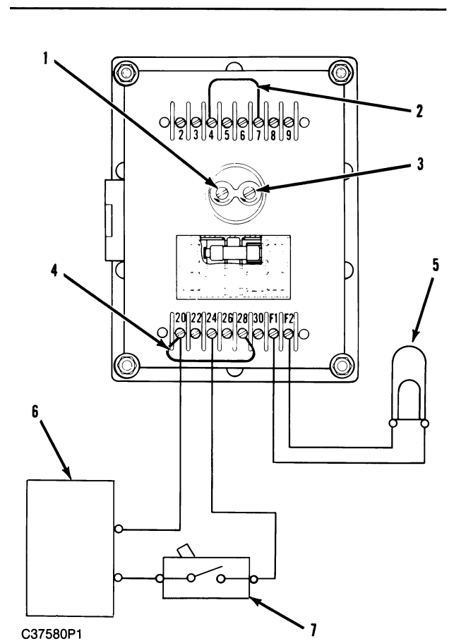
Bench Test Circuit
