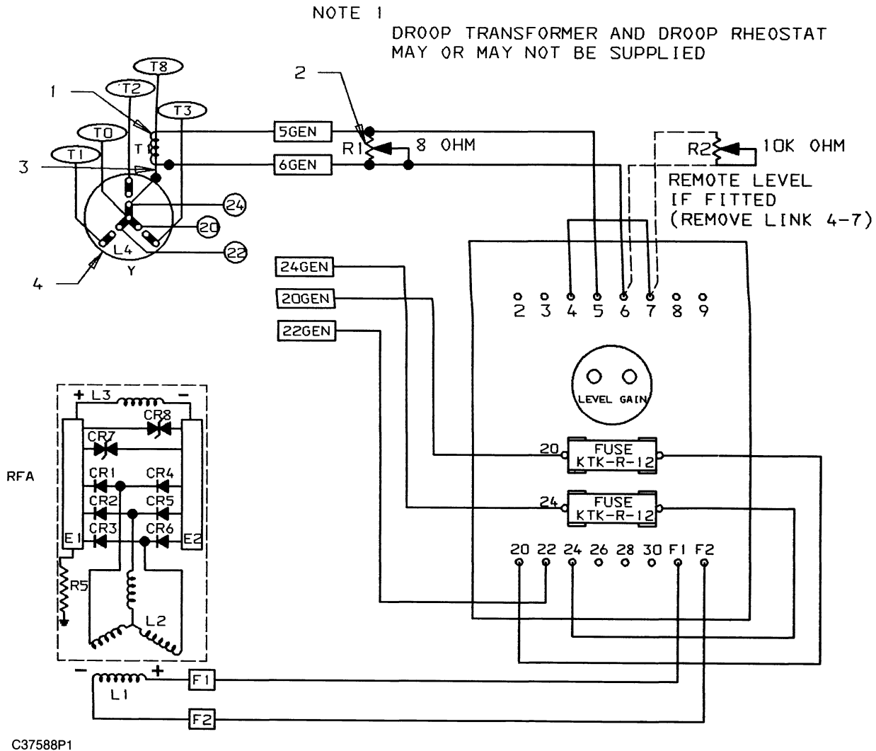
Generator And Regulator Schematic (1) Voltage droop transformer. (2) Voltage droop rheostat. (3) Lead. (4) Main stator.
