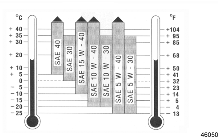
Figure 3-1 Operating Ranges for SAE Viscosity Grades
