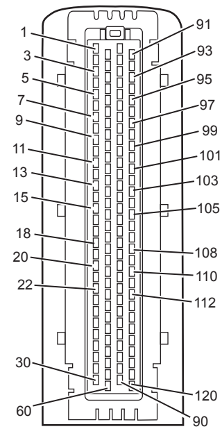
120-PIN CONNECTOR
