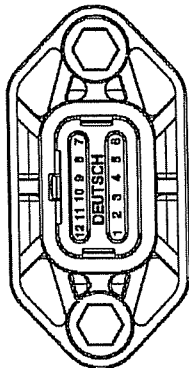
WIRE INSERTION VIEW
