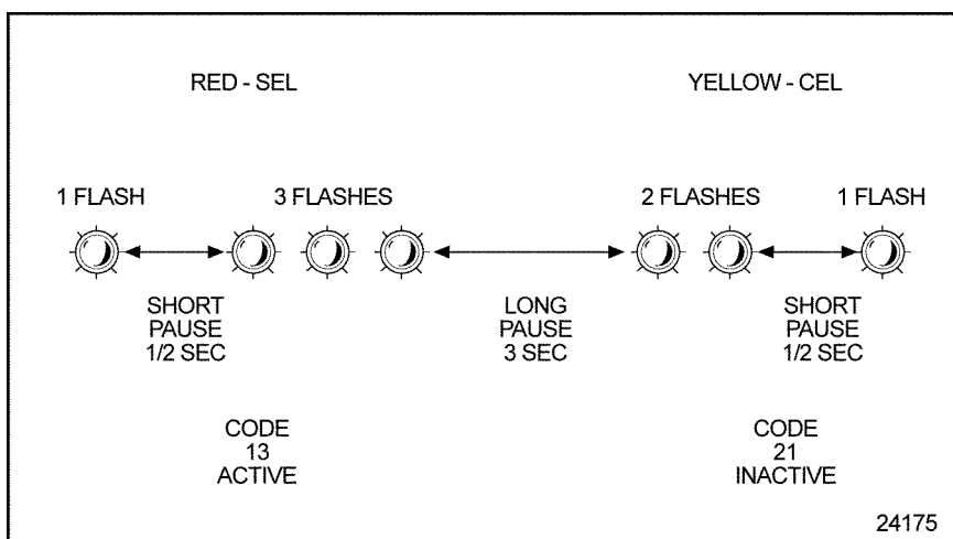
Figure 5-6 Flash Codes
