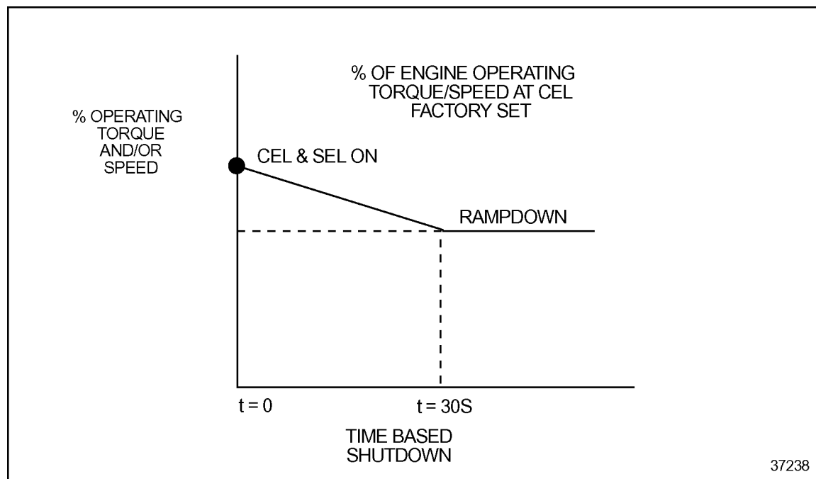
Figure 5-11 Rampdown
