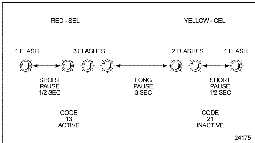
Figure 7-1 Flash Codes
