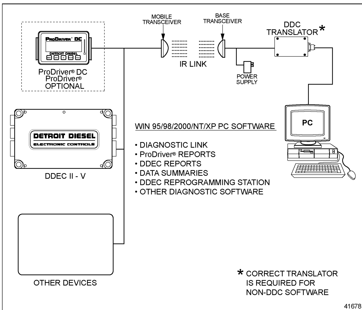
Figure 5-36 IRIS Configuration
