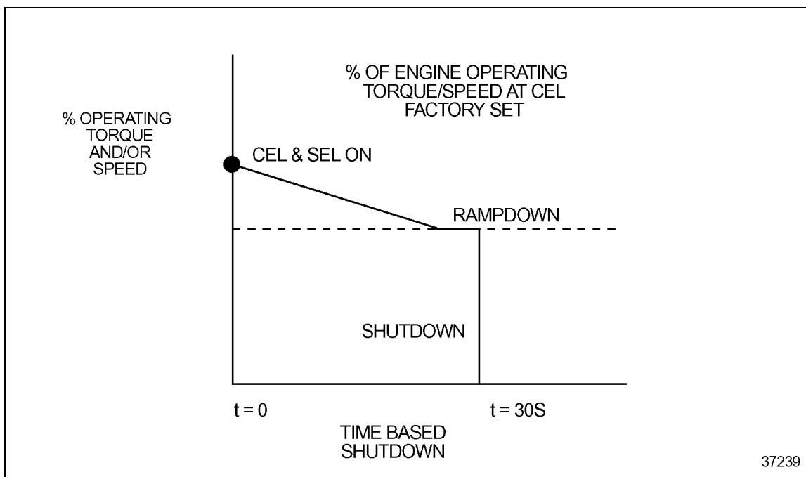
Figure 5-12 Engine Shutdown
