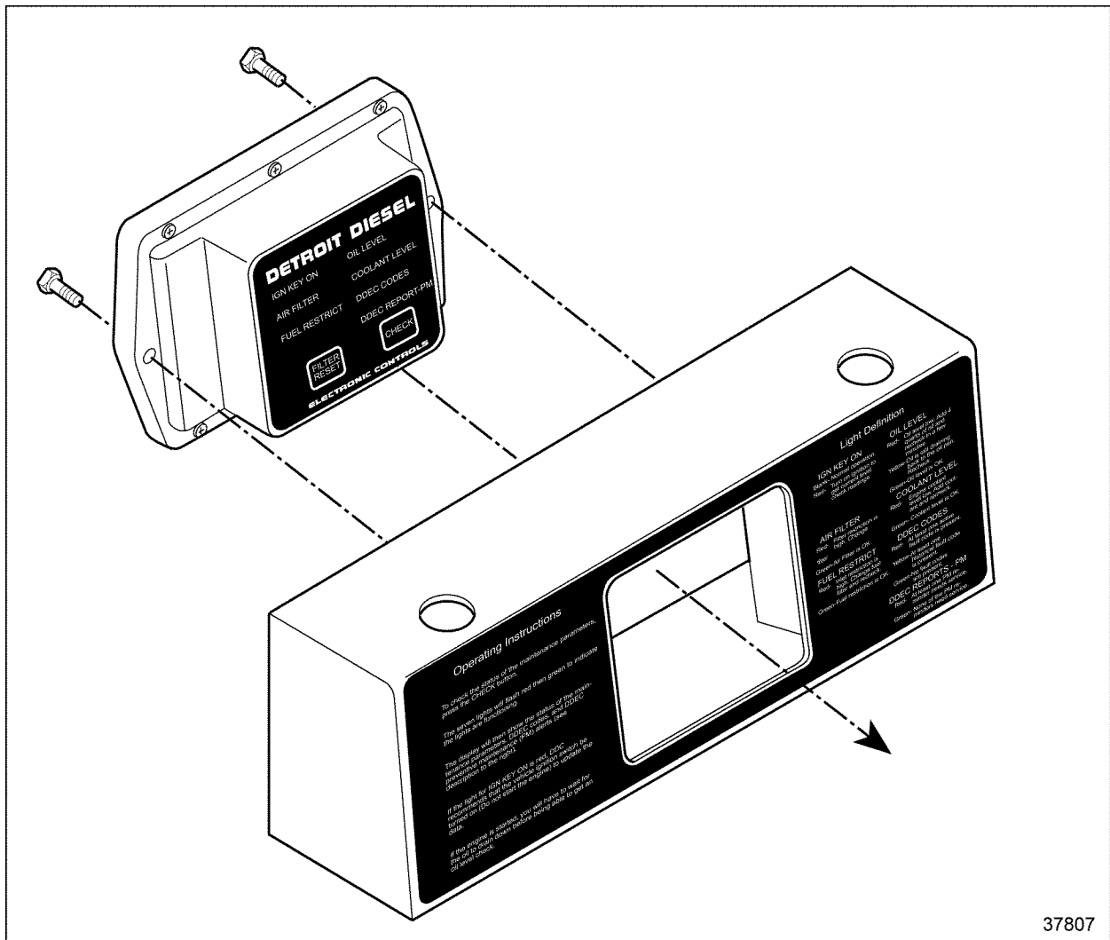
Figure 5-54 Maintenance Alert Display and Bracket
