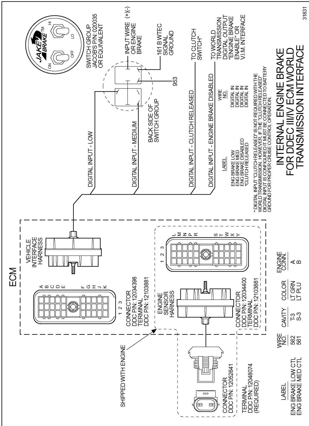
Figure 5-10 Internal Engine Brake for DDEC IV ECM World Transmission Interface
