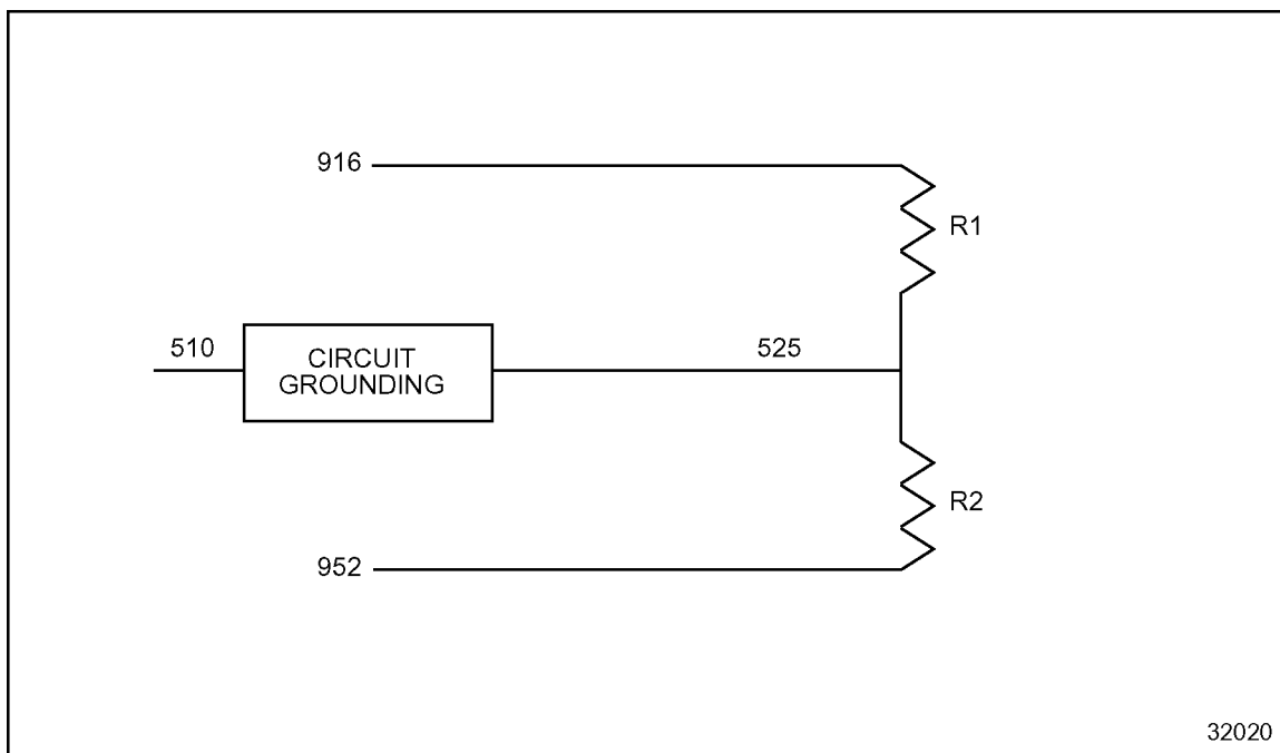
Figure 5-81 Voltage Divider
