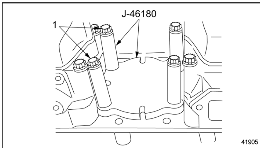
Figure 4 Measuring Plate Installation
