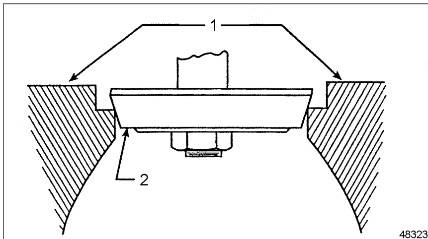
1. Cylinder Block
