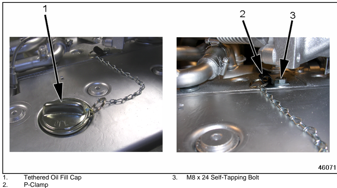
Figure 1 Identification of Installed Tethered Oil Fill Cap Kit (pre-EPA07)
