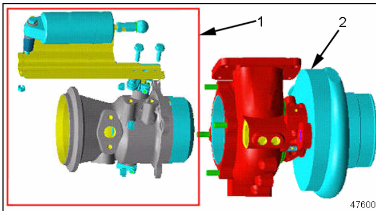
Figure 12 Turbo Brake Assembly
