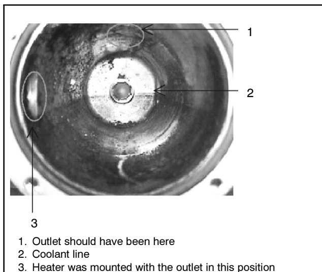
Figure 6 Improper Heater Mounting Position
