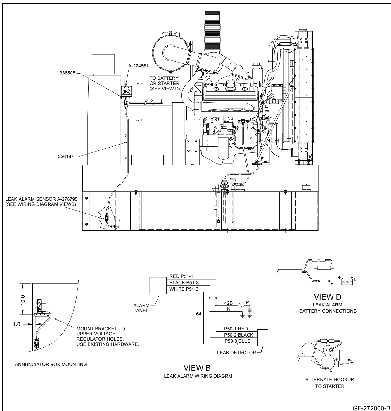
Figure 1. 200-400 kW Double-Wall Subbase Fuel Tank Leak Alarm
