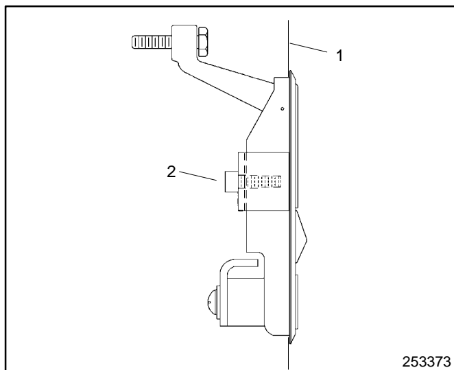
Figure 2. Door Latch
