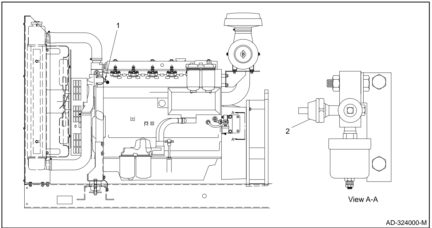
Figure 1. Plug Removal and Switch Installation Locations
