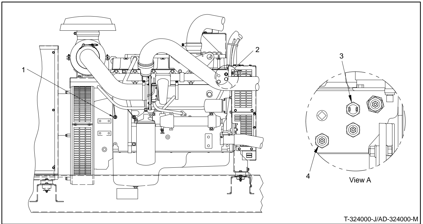
Figure 1. Plug Removal and Switch Installation Locations (150/180 kW shown)
