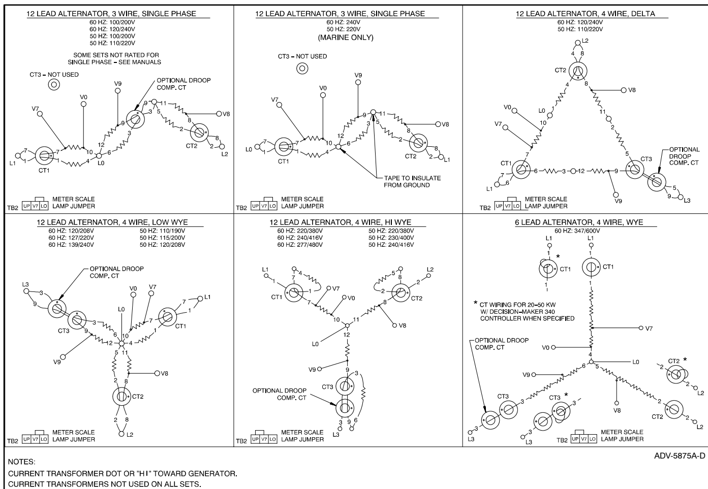
Figure 3 Generator Connections
