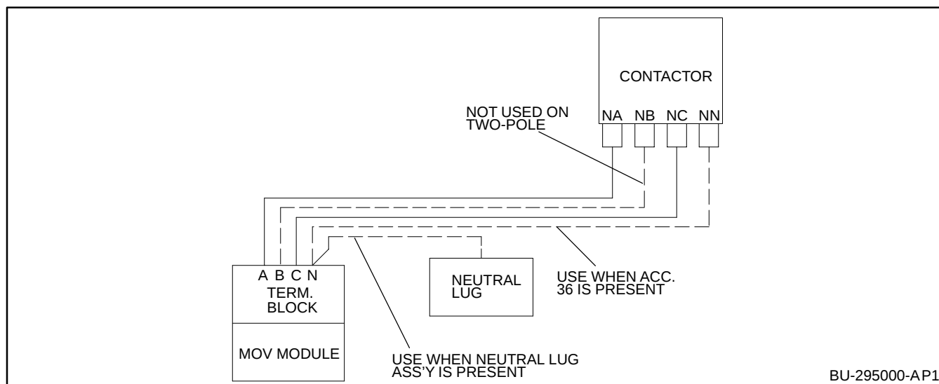
Figure 5. Wiring Diagram—600-800 Amp
