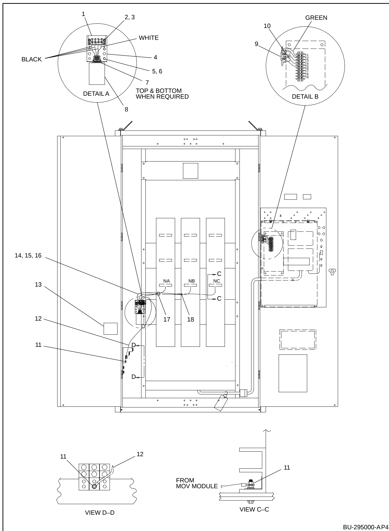
Figure 12. Assembly—3000-4000 Amp
