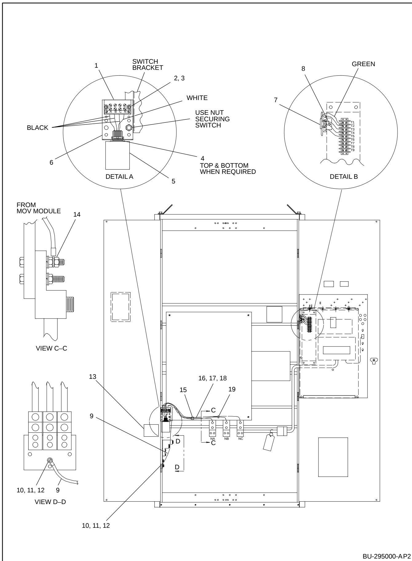
Figure 8. Assembly—1000-1200 Amp
