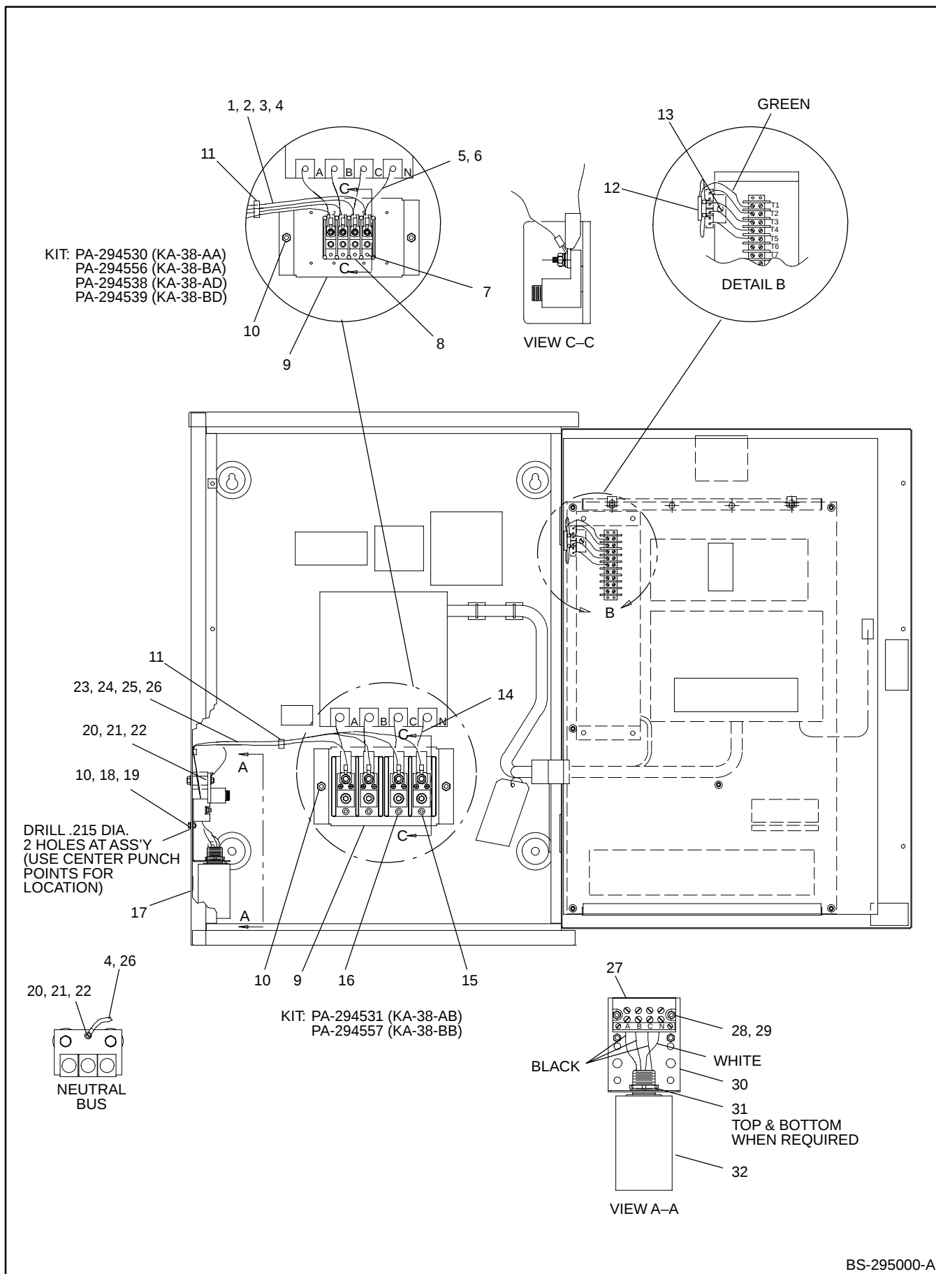
Figure 3. Assembly—30-104, 150 Amp
