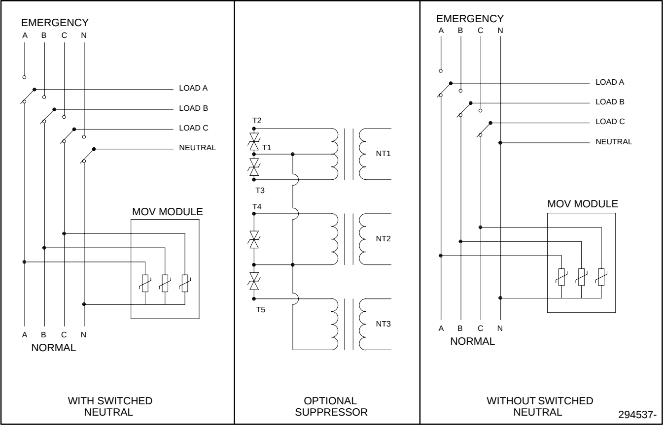
Figure 11. Schematic Diagram
