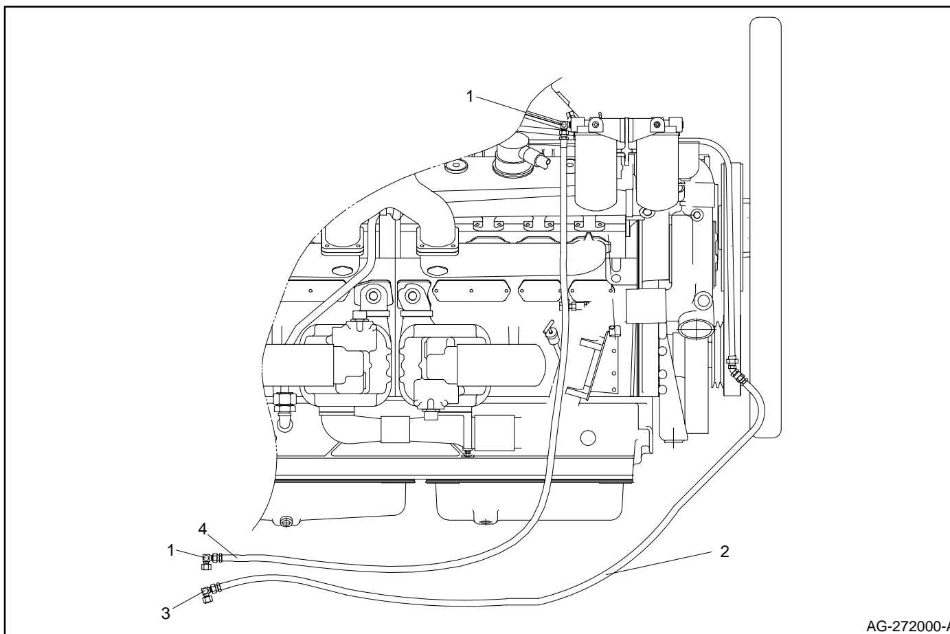
Figure 1. Flexible Fuel Line Connections
