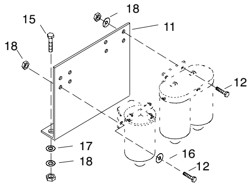
Fuel Filter Mounting Bracket And Hardware
