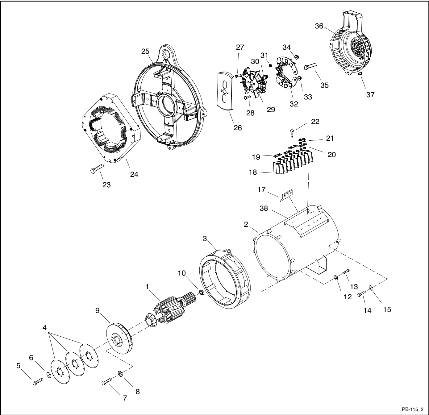
Figure 2 Alternator Drawing
