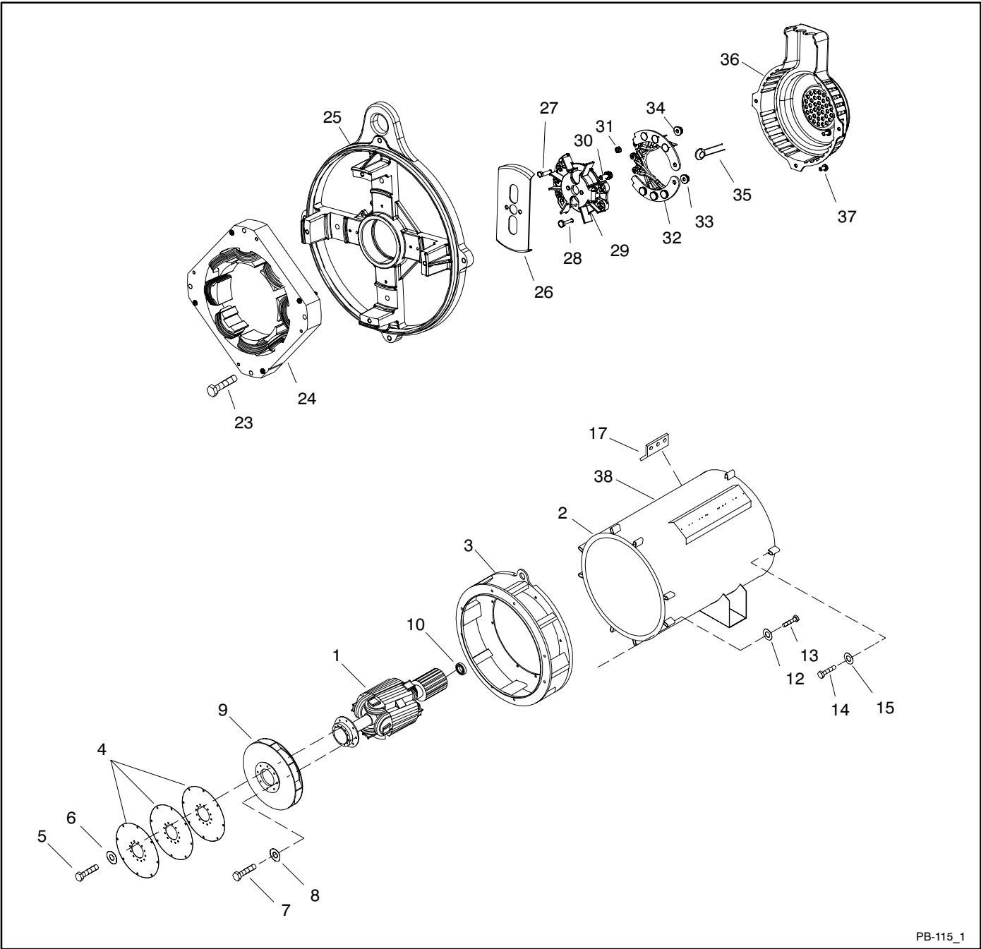
Figure 1 Alternator Drawing
