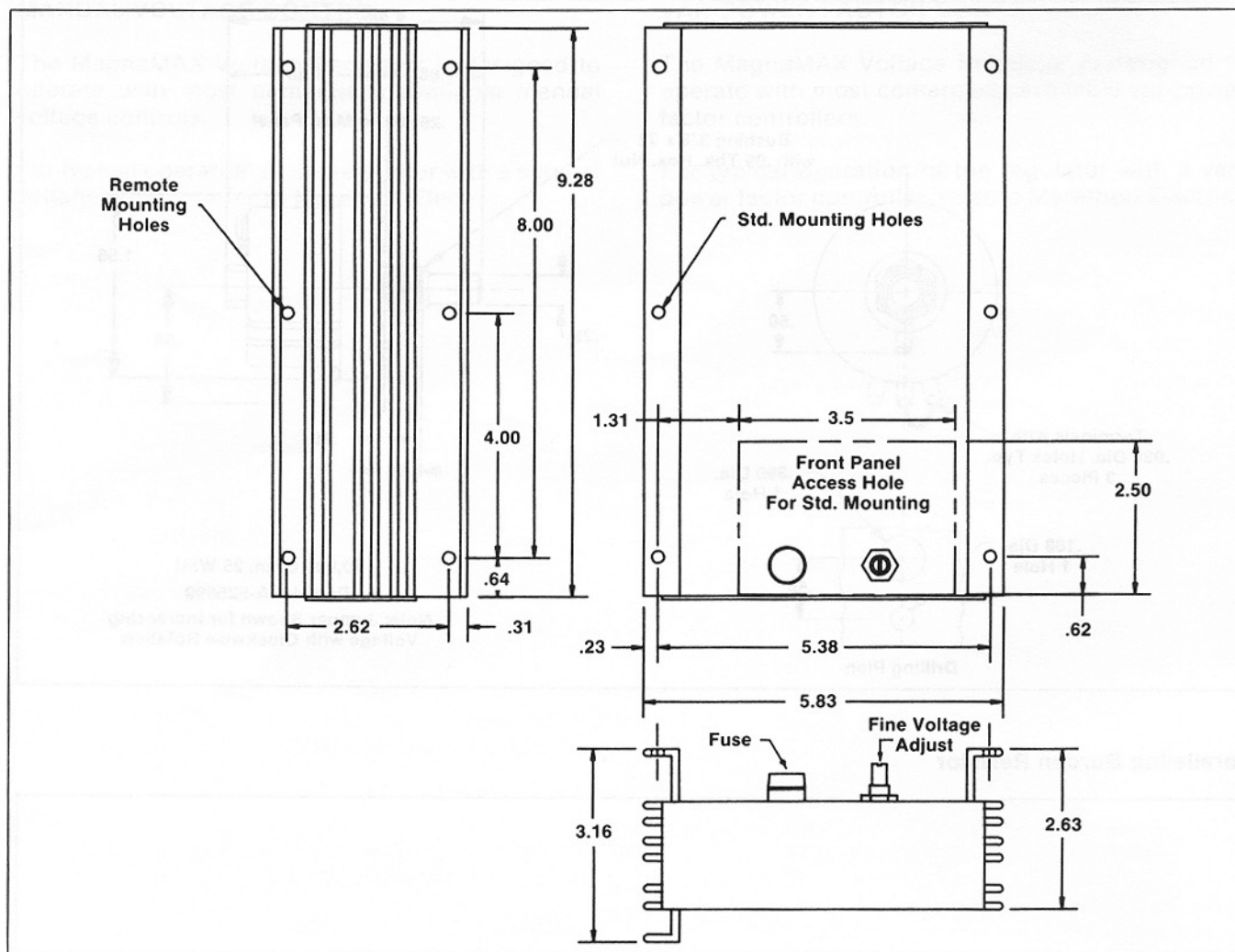
Outline Drawing of Regulator
