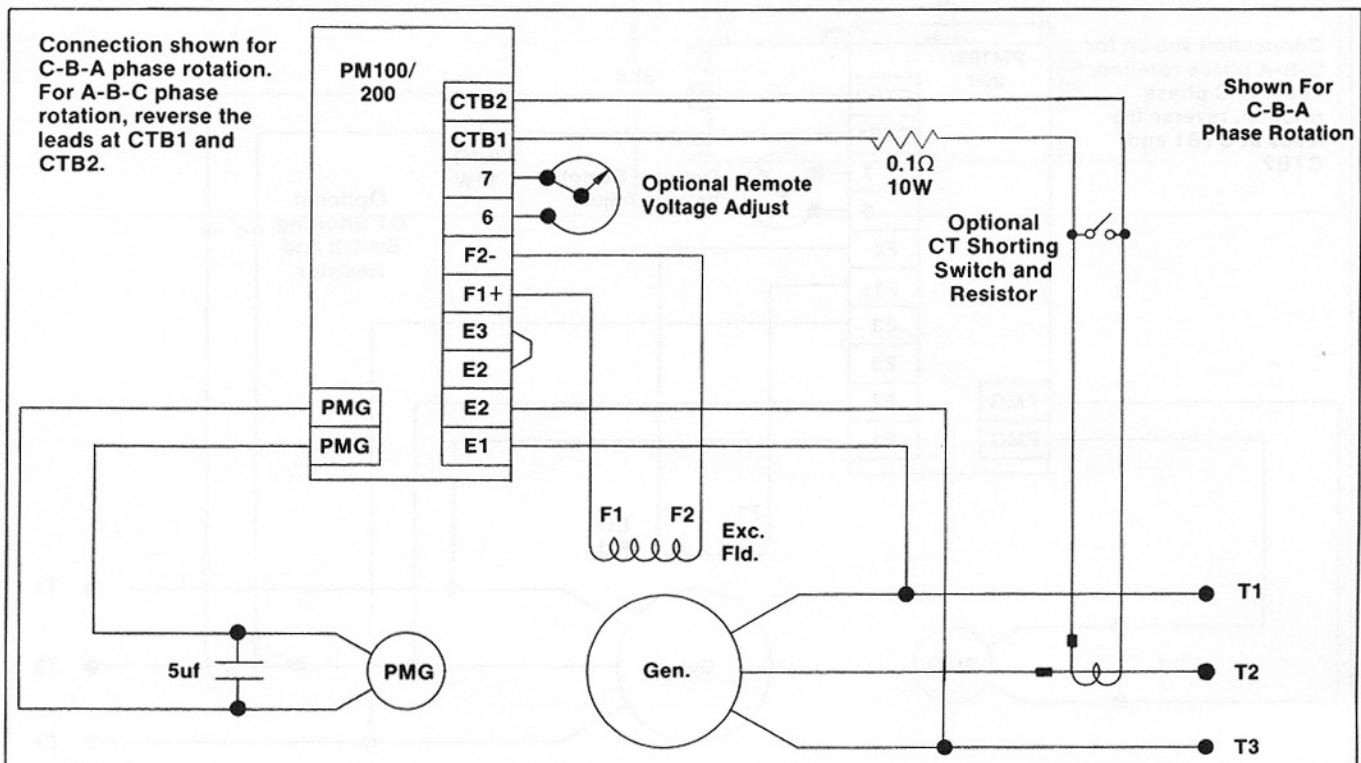
Typical Connection - Single Phase Sensing (95-600 Volts) with Reactive Droop Paralleling
