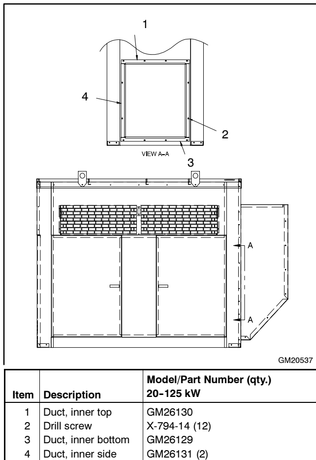
Figure 2 Installing the Inner Duct Components
