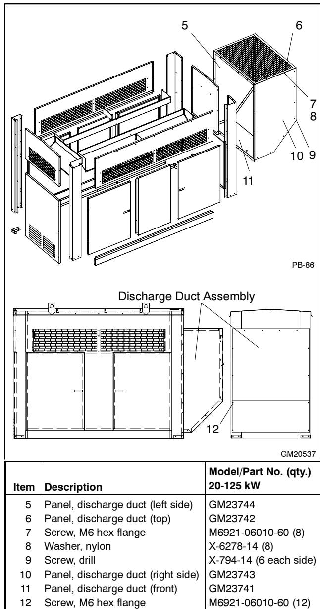
Figure 4 Assembling the Discharge Duct
