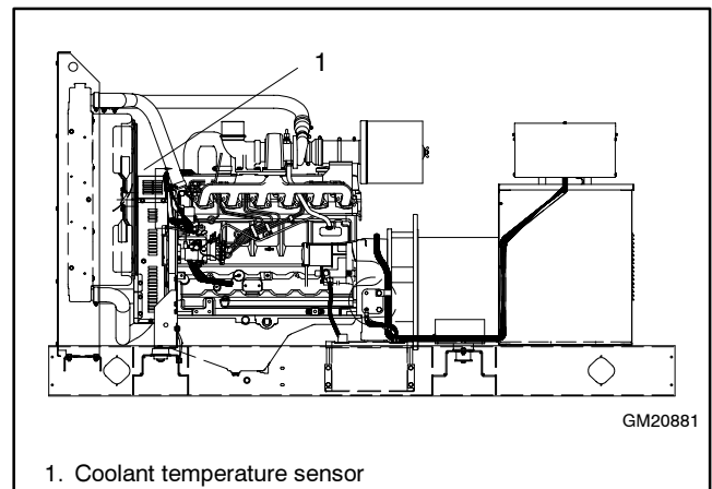
Figure 3 Coolant Temperature Sender Location, Typical
