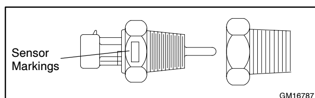
Figure 1 Coolant Temperature Sensor and Reducer Bushing (if equipped), Typical
