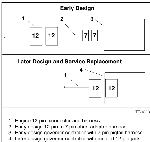
Figure 1 Governor Controller Configurations
