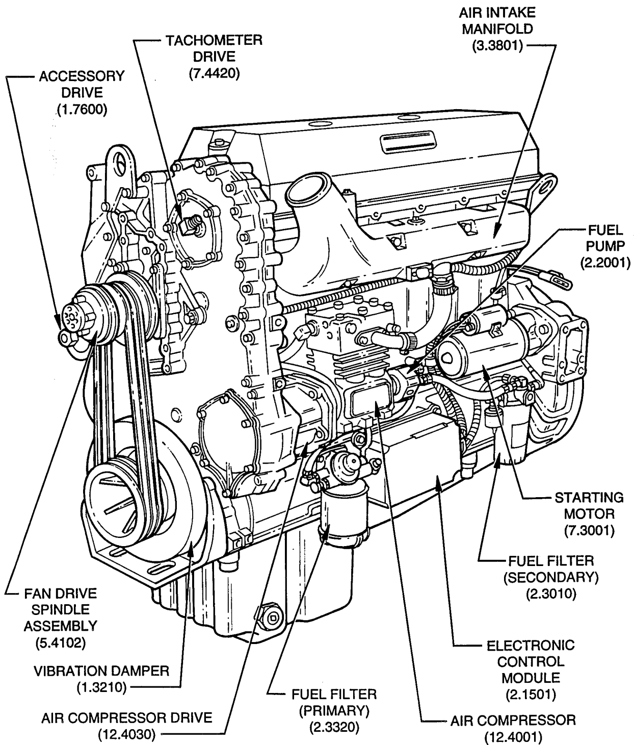
TYPICAL SERIES 60 ENGINE
