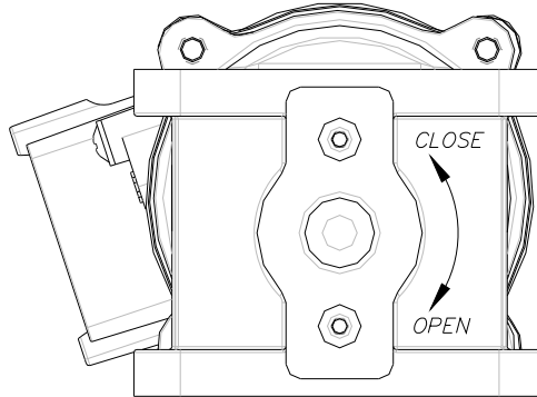
Figure 3-1. Spring-loaded Throttle Plate
